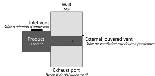
Figure 1. Schematic of the installation of the product.
