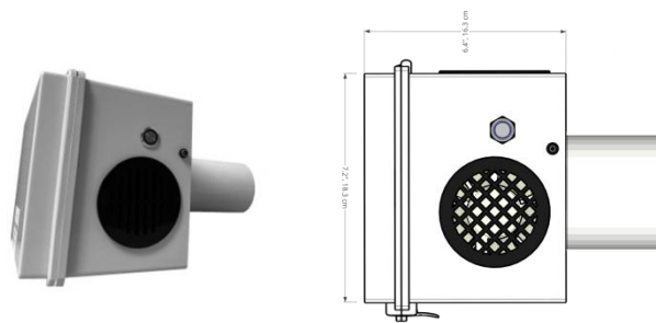
The length of the exhaust port is ~6.5" (165 mm) | The length of the complete unit is ~13" (330 mm)
